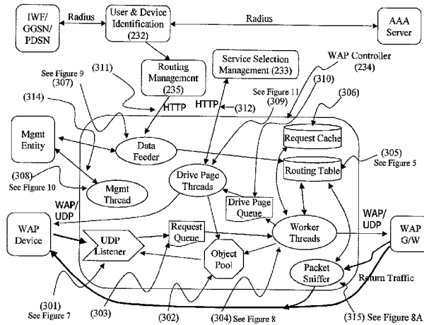
WAP Controller (234) Block Diagram
