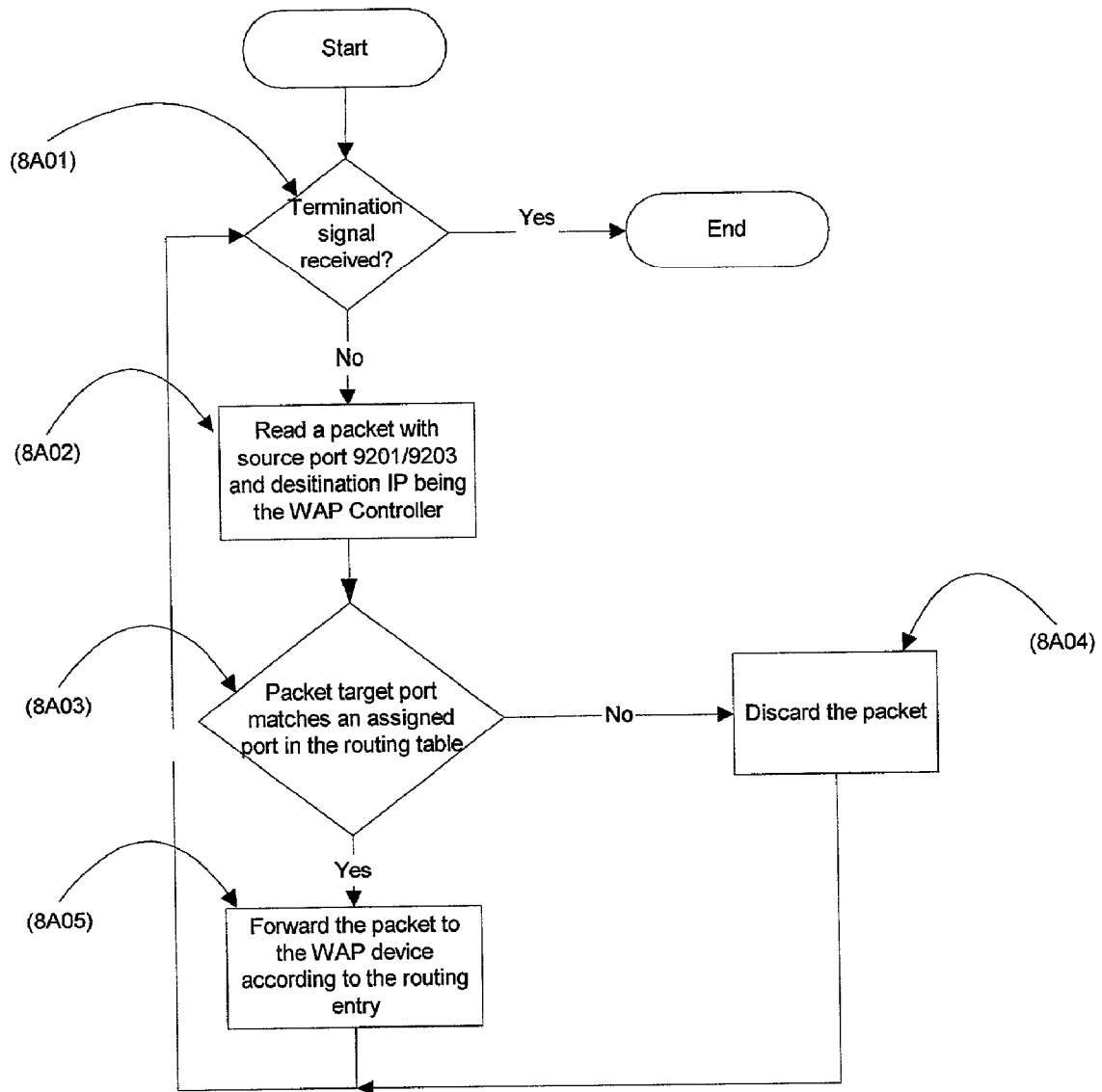
Figure 8A Flow Chart of Packet Sniffer Thread (315)
