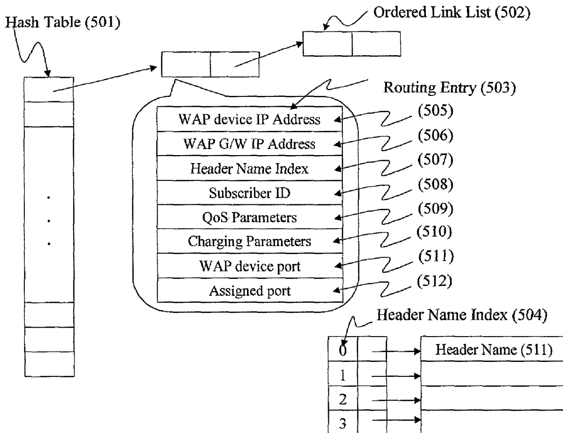
Figure 5 WAP Controller (234) Routing Table (305) Data Structure
